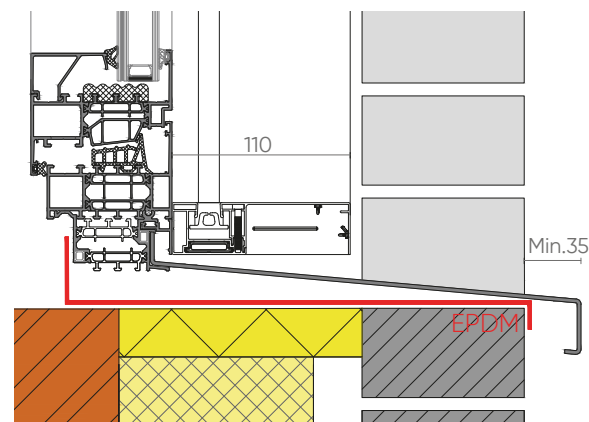
RAAMDORPEL + SCREENGLEIDER INTEGRATED
